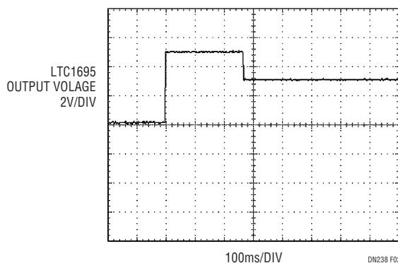
Figure 2. Fan Start-Up Voltage Profile
